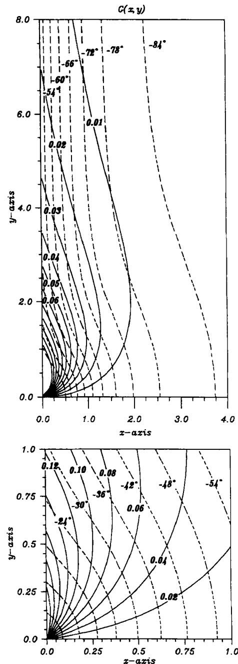
Figure 3 Amplitude- (solid lines) and phase- (dashed lines) level lines of G(x, y)
